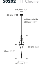
50201 H1 Gold balls 50202 H1 Chrome balls
