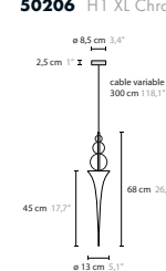
50205 H1 XL Gold balls 50206 H1 XL Chrome balls
