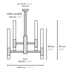
16558 H12+12 XL Clear Glass 17558 H12+12 XL Frosted Glass
