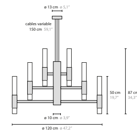
16565 H17+17 Clear Glass 17565 H17+17 Frosted Glass
