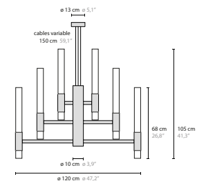
16567 H17+17 XL Clear Glass 17567 H17+17 XL Frosted Glass
