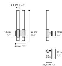
14525 W2+2 XL Clear Glass 15525 W2+2 XL Frosted Glass
