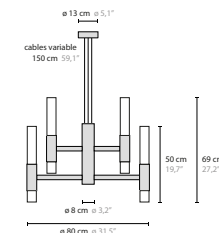
16557 H12+12 Clear Glass 17557 H12+12 Frosted Glass
