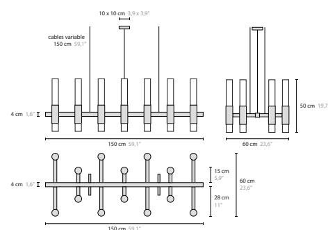
16576 H14+14 cross Clear Glass 17576 H14+14 cross Frosted Glass
