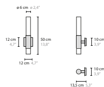
16519 W1+1 Clear Glass 17519 W1+1 Frosted Glass
