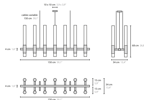
16577 H14+14 cross XL Clear Glass 17577 H14+14 cross XL Frosted Glass
