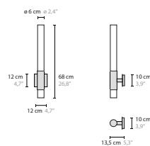
14521 W1+1 XL Clear Glass 15521 W1+1 XL Frosted Glass
