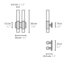
16523 W2+2 Clear Glass 17523 W2+2 Frosted Glass
