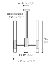
16554 H6+6 XL Clear Glass 17554 H6+6 XL Frosted Glass
