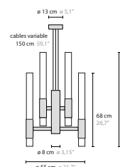
16556 H9+9 XL Clear Glass 17556 H9+9 XL Frosted Glass
