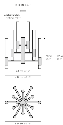
16563 H15+15 XL Clear Glass 17563 H15+15 XL Frosted Glass
